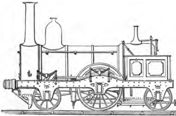
Fig. 109.—Midland Railway. No. 60, built April, 1848, by Sharp Brothers (for details see p. 103).
